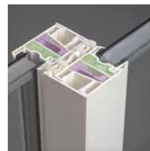
FiberCore™ structural meeting rail stiles for added strength, UltraCore™ insulation for enhanced efficiency and our exclusive Clash Free Interlock.
