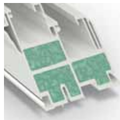
UltraCore™ polyurethane insulated windows offer higher resistance to heat and cold providing you with added comfort.
